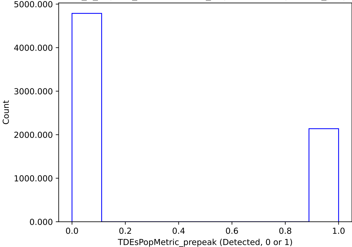
internal_u_expt30_nscale1.2v3.4_10yrs : TDEsPopMetric_prepeak
