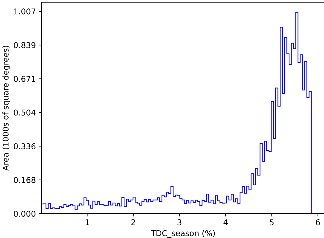
internal_u_expt30_nscale1.2v3.4_10yrs : TDC_season
