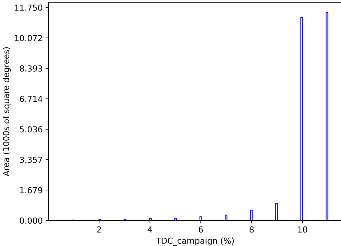
internal_u_expt30_nscale1.2v3.4_10yrs : TDC_campaign
