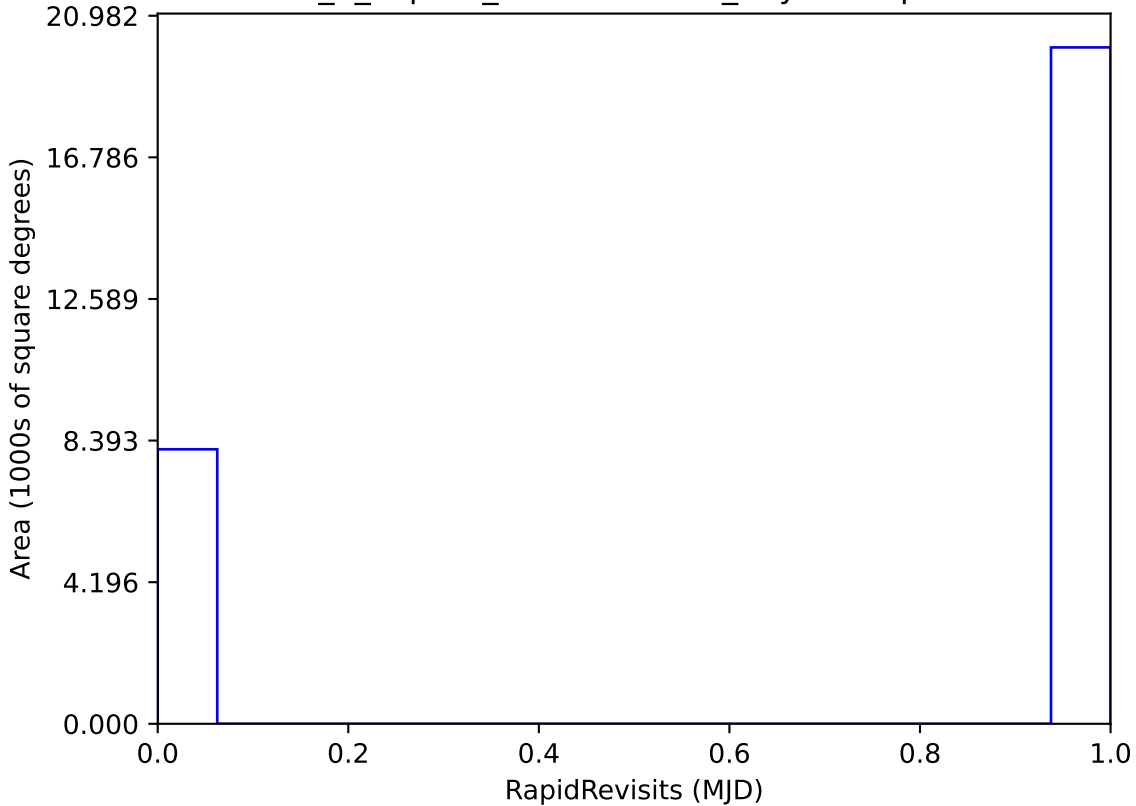
internal_u_expt30_nscale1.2v3.4_10yrs : RapidRevisits
