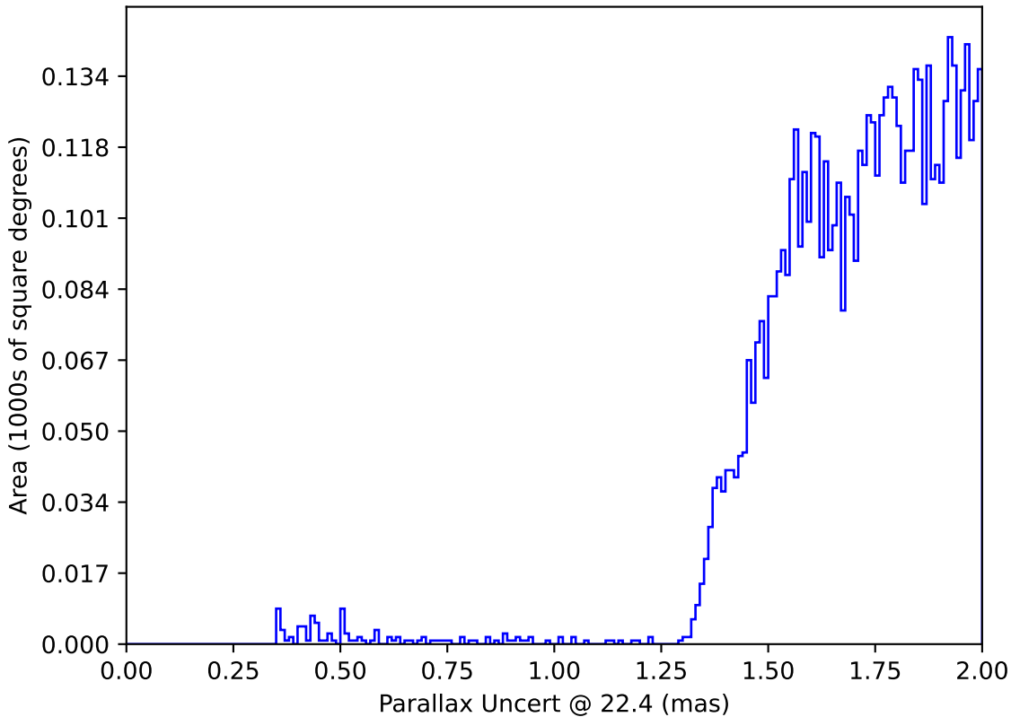
internal_u_expt30_nscale1.2v3.4_10yrs : Parallax Uncert @ 22.4
