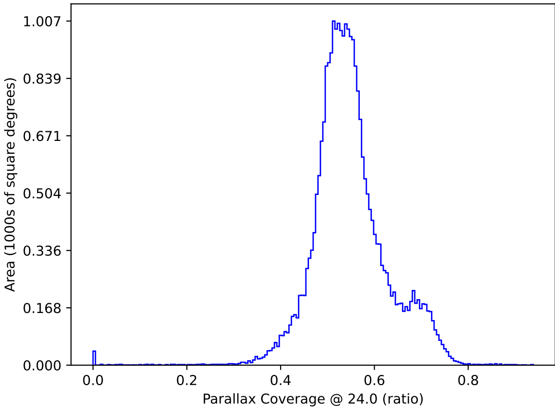
internal_u_expt30_nscale1.2v3.4_10yrs : Parallax Coverage @ 24.0
