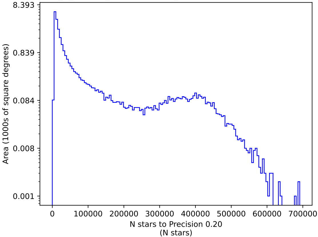
internal_u_expt30_nscale1.2v3.4_10yrs z: N stars to Precision 0.20
