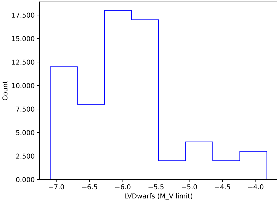
internal_u_expt30_nscale1.2v3.4_10yrs gi: LVDwarfs
