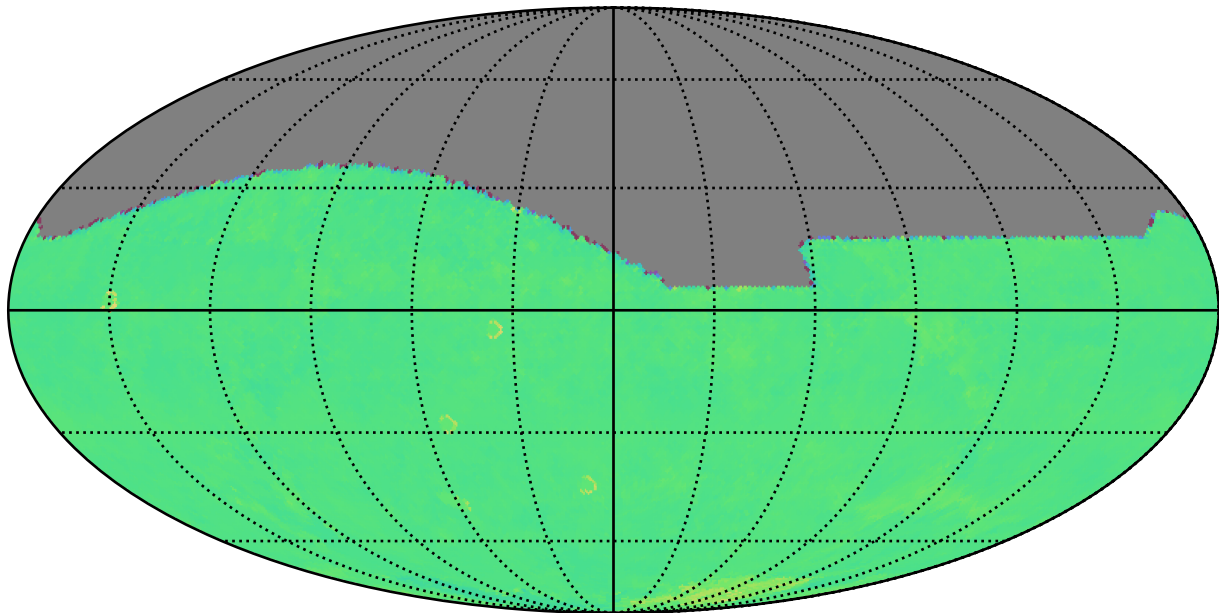
internal_u_expt30_nscale1.2v3.4_10yrs r: Kuiper rotTelPos
