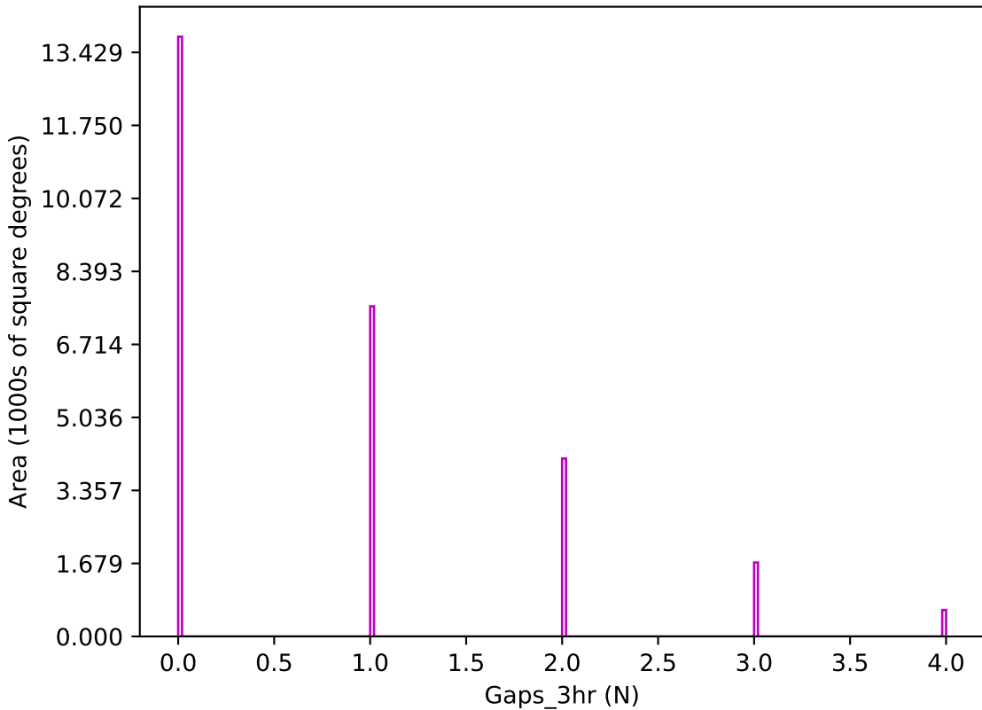
internal_u_expt30_nscale1.2v3.4_10yrs z band: Gaps_3hr
