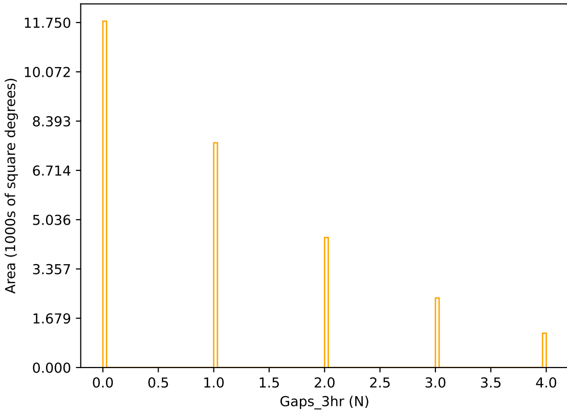
internal_u_expt30_nscale1.2v3.4_10yrs r band: Gaps_3hr
