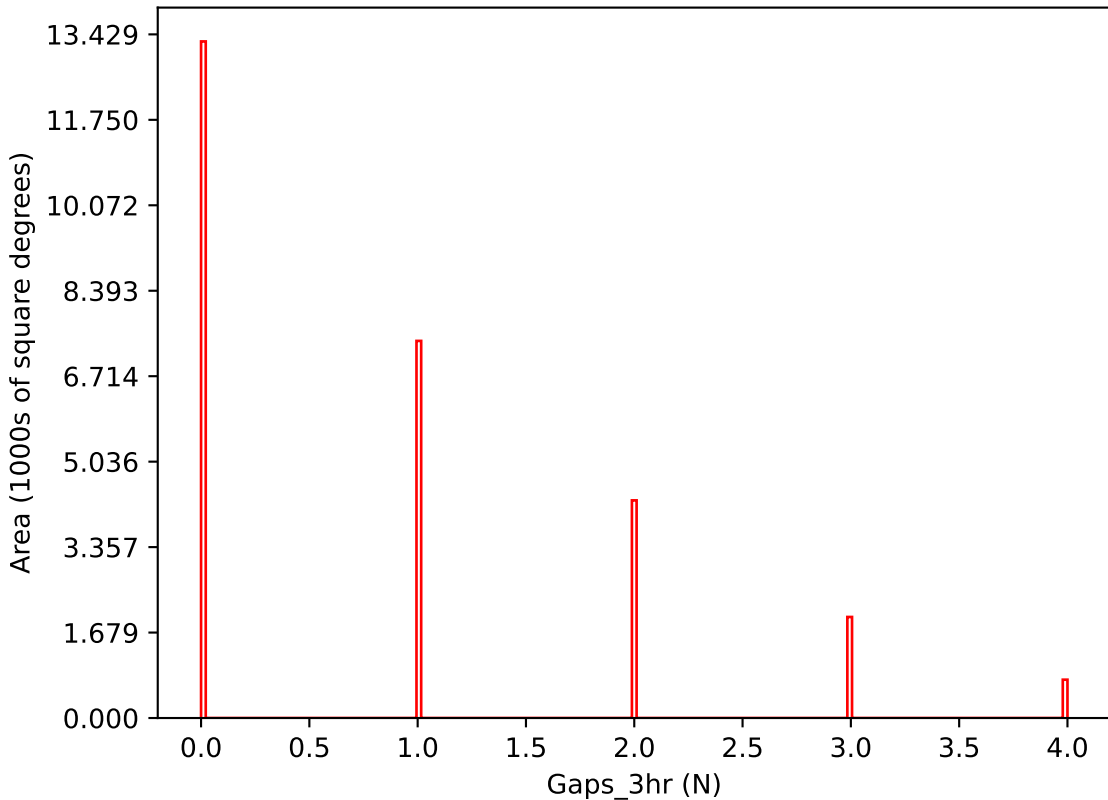
internal_u_expt30_nscale1.2v3.4_10yrs i band: Gaps_3hr
