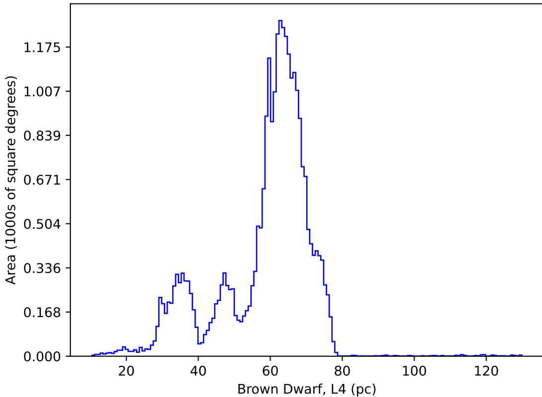
internal_u_expt30_nscale1.2v3.4_10yrs : Brown Dwarf, L4
