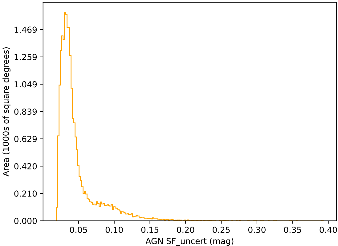
internal_u_expt30_nscale1.2v3.4_10yrs r band: AGN SF_uncert
