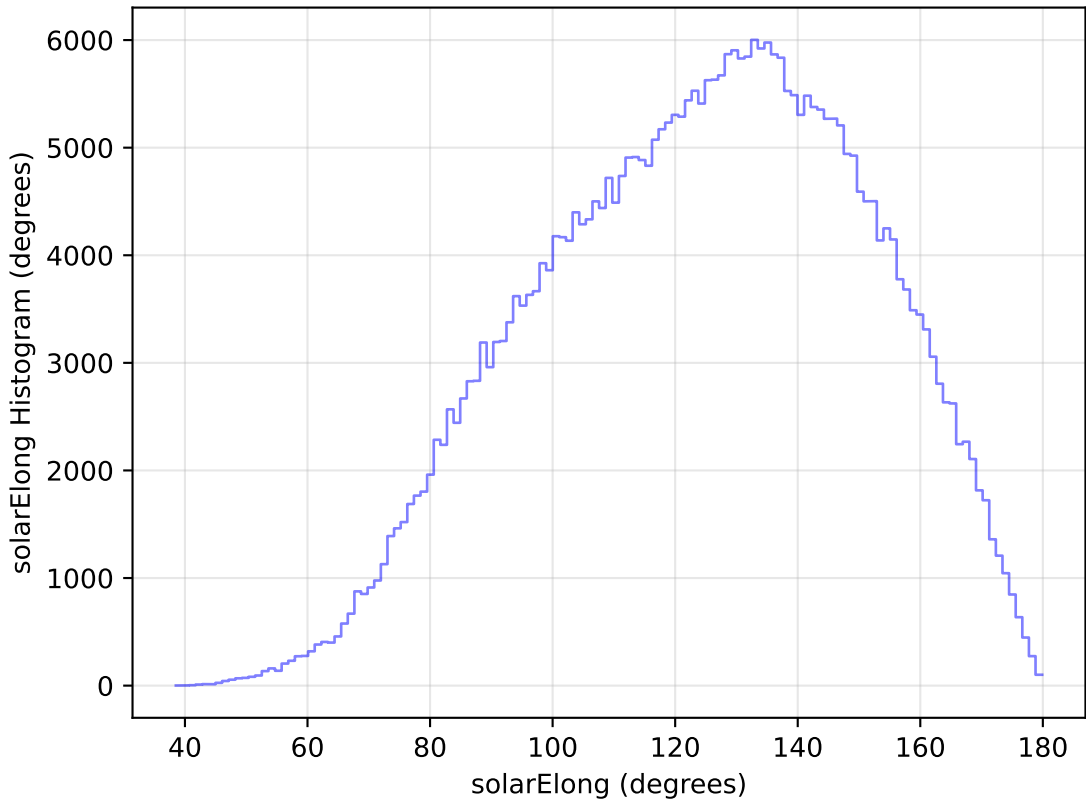
internal_u_expt30_nscale1.2v3.4_10yrs WFD y band: solarElong Histogram
