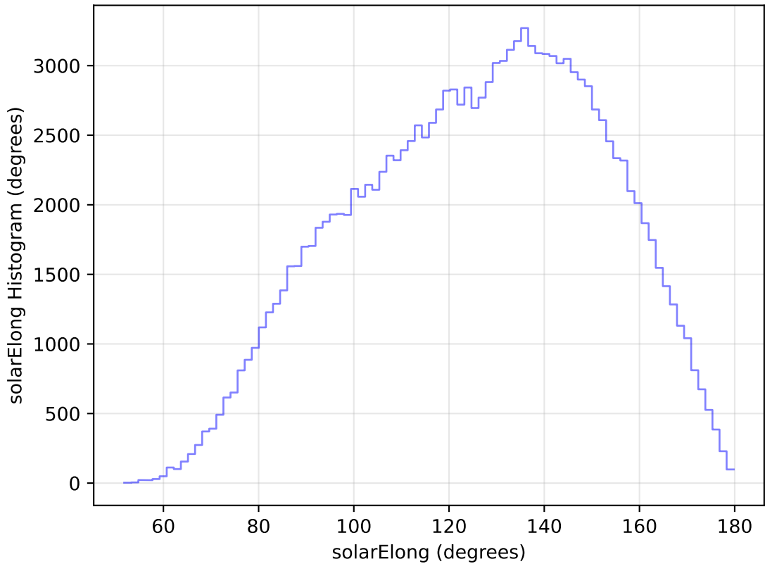
internal_u_expt30_nscale1.2v3.4_10yrs WFD u band: solarElong Histogram
