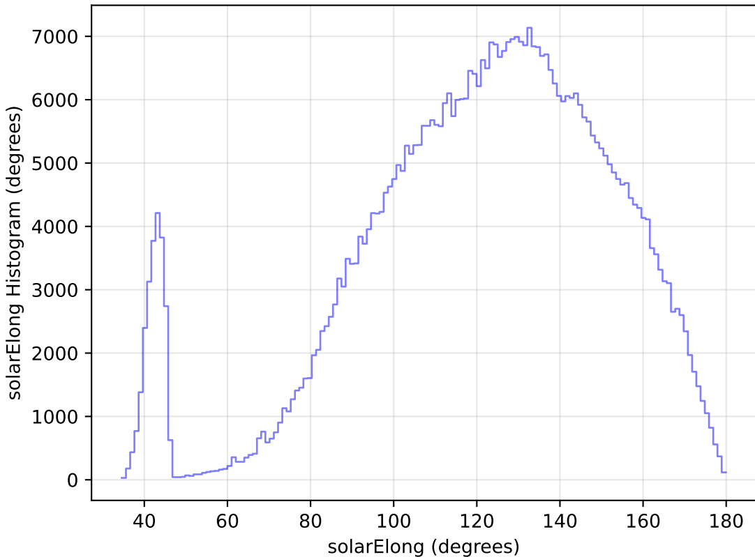
internal_u_expt30_nscale1.2v3.4_10yrs WFD i band: solarElong Histogram
