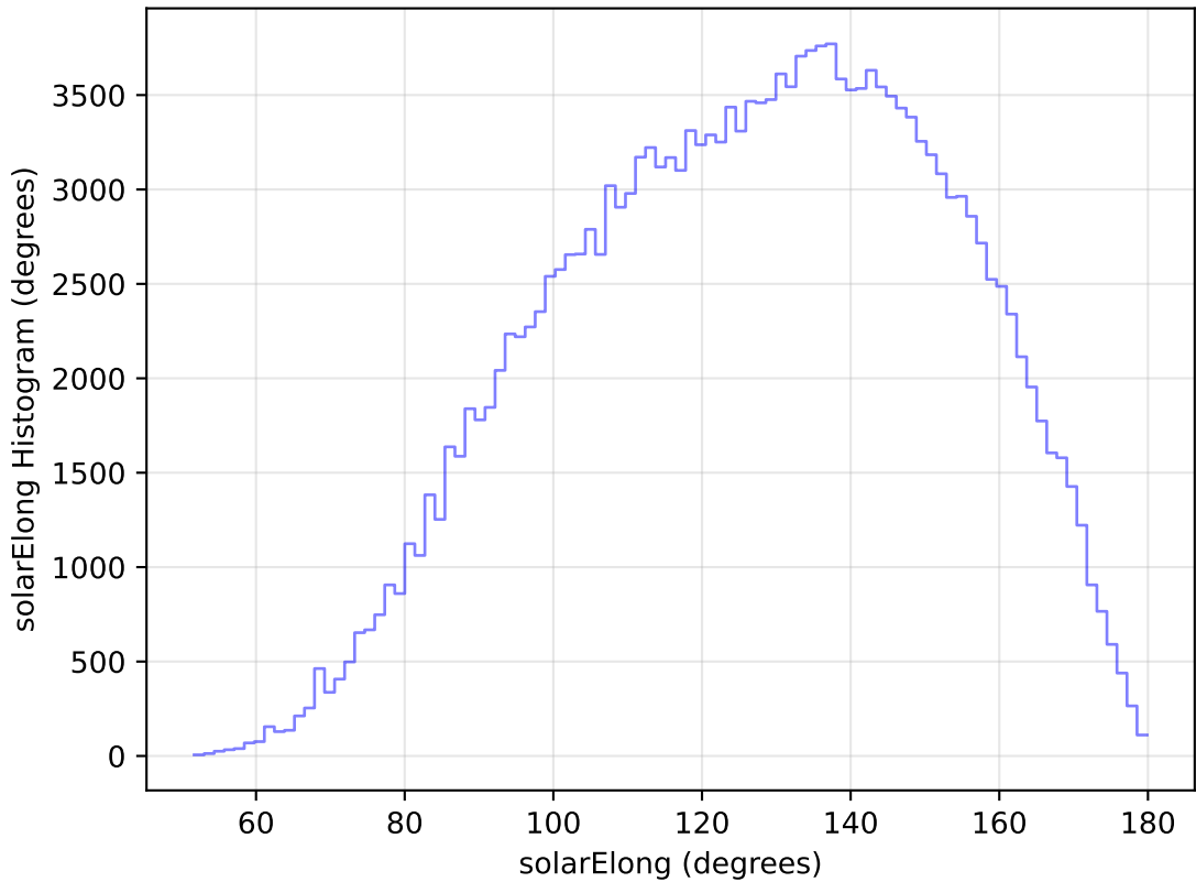
internal_u_expt30_nscale1.2v3.4_10yrs WFD g band: solarElong Histogram
