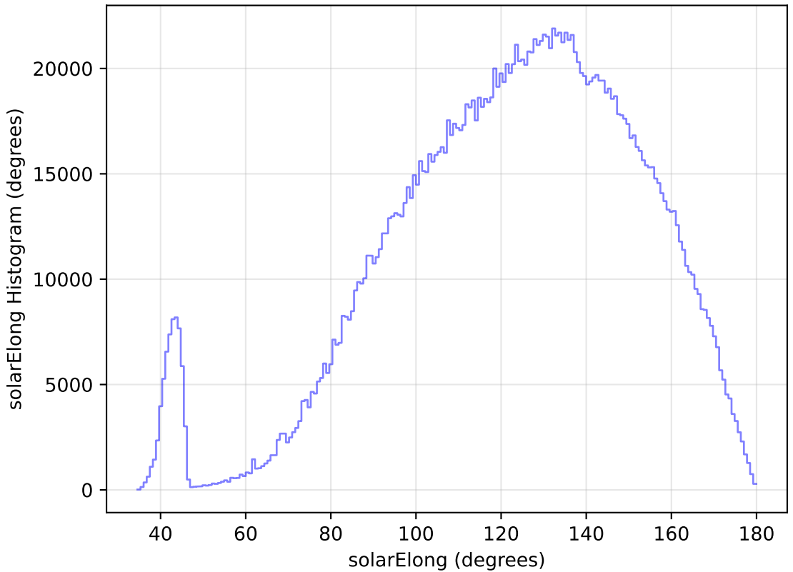
internal_u_expt30_nscale1.2v3.4_10yrs WFD all bands: solarElong Histogram
