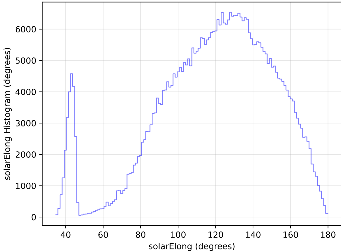
internal_u_expt30_nscale1.2v3.4_10yrs All sky z band: solarElong Histogram
