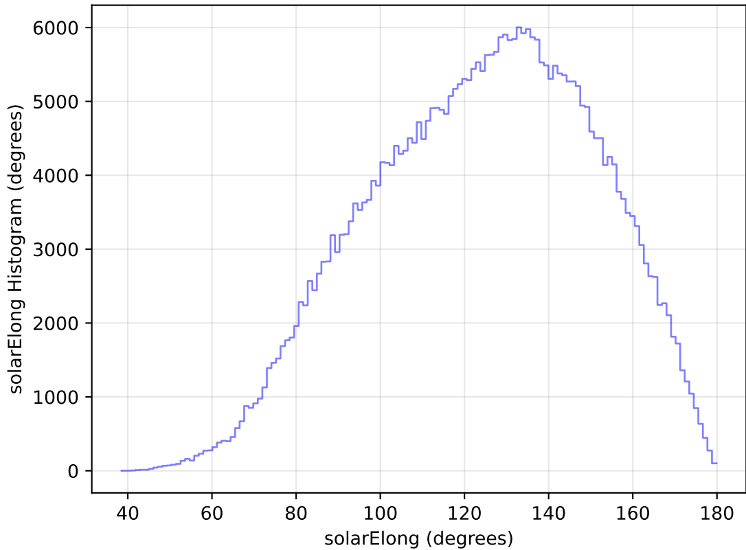
internal_u_expt30_nscale1.2v3.4_10yrs All sky y band: solarElong Histogram
