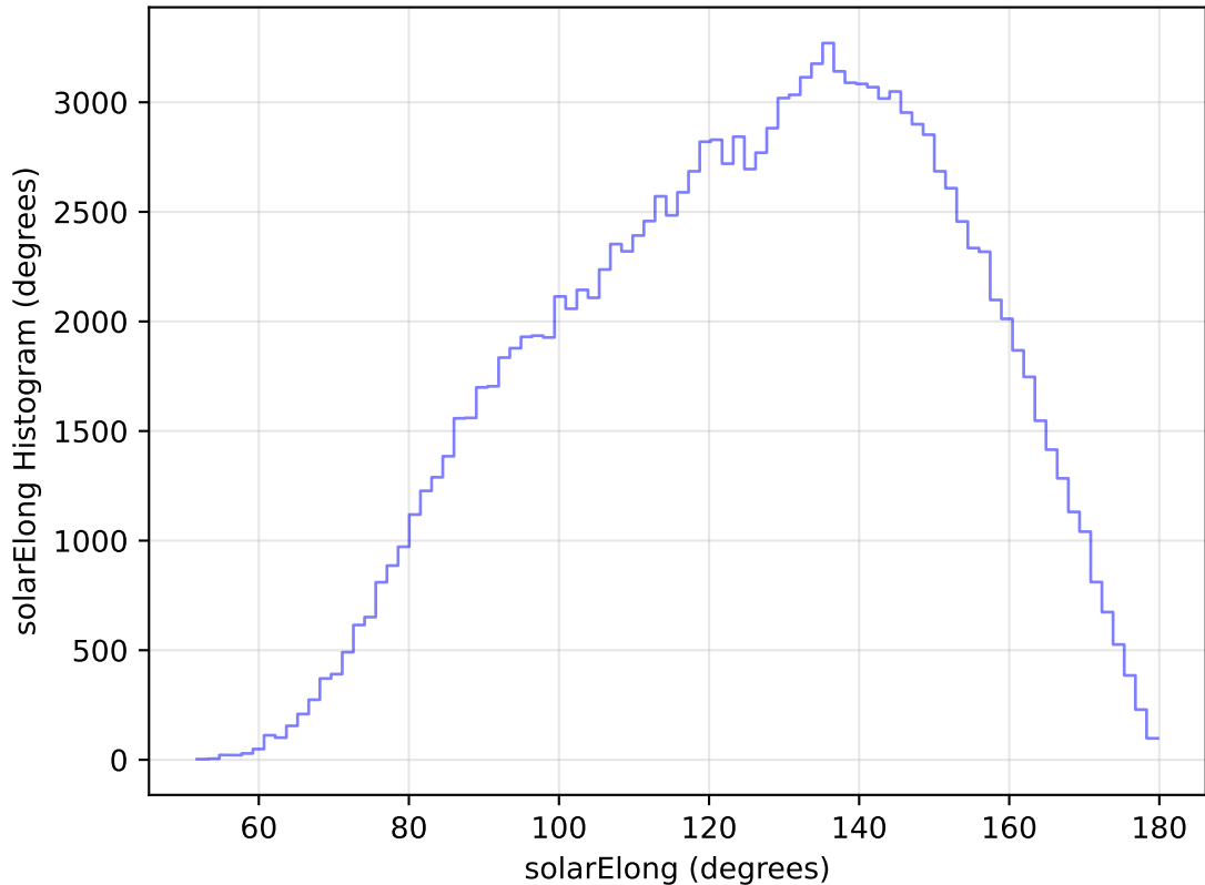
internal_u_expt30_nscale1.2v3.4_10yrs All sky u band: solarElong Histogram
