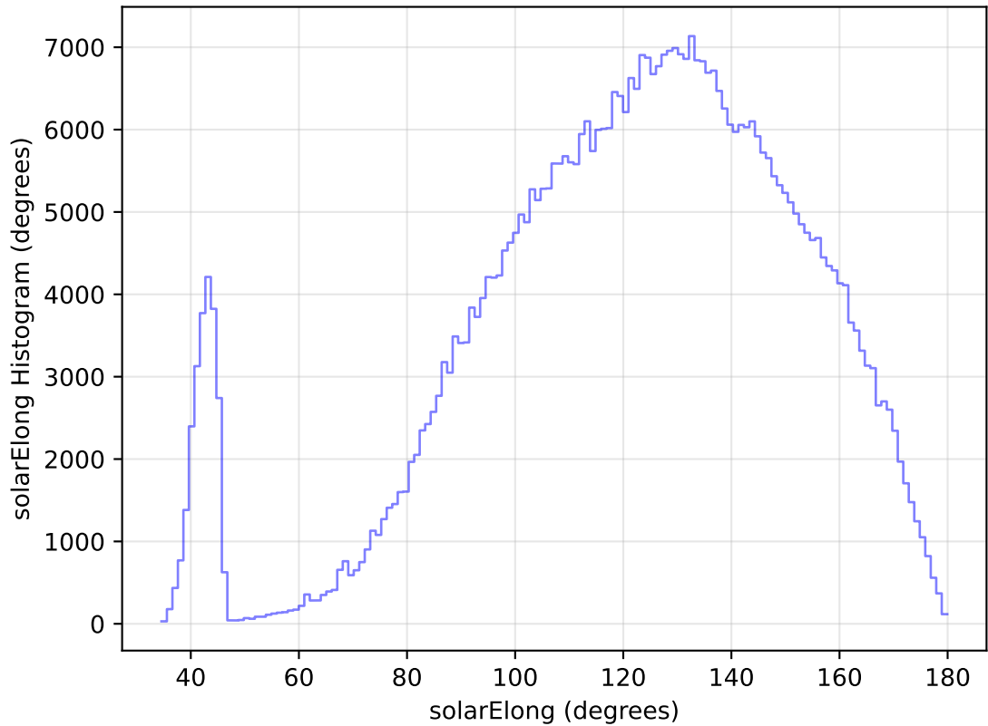
internal_u_expt30_nscale1.2v3.4_10yrs All sky i band: solarElong Histogram
