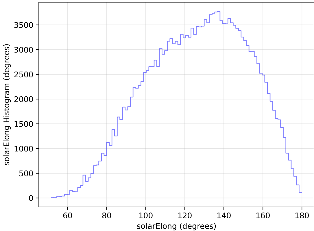
internal_u_expt30_nscale1.2v3.4_10yrs All sky g band: solarElong Histogram
