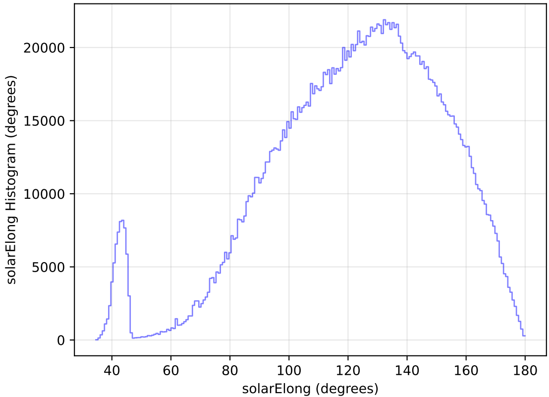
internal_u_expt30_nscale1.2v3.4_10yrs All sky all bands: solarElong Histogram
