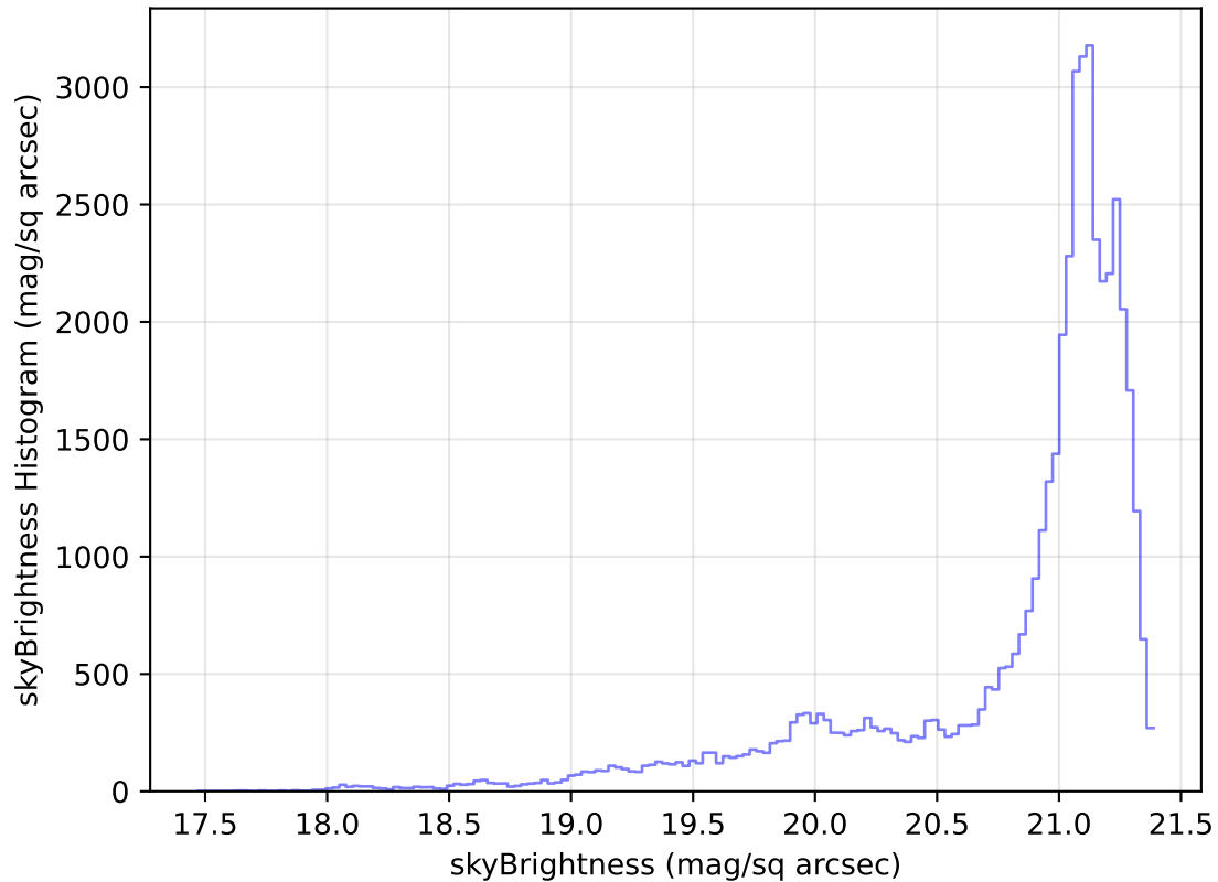
internal_u_expt30_nscale1.2v3.4_10yrs Yr 1 r band: skyBrightness Histogram
