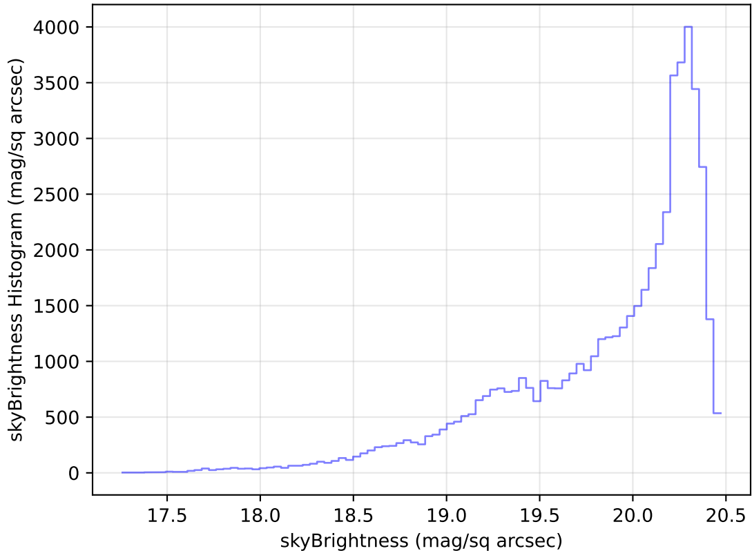
internal_u_expt30_nscale1.2v3.4_10yrs Yr 1 i band: skyBrightness Histogram
