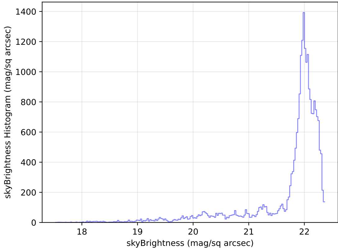
internal_u_expt30_nscale1.2v3.4_10yrs Yr 1 g band: skyBrightness Histogram
