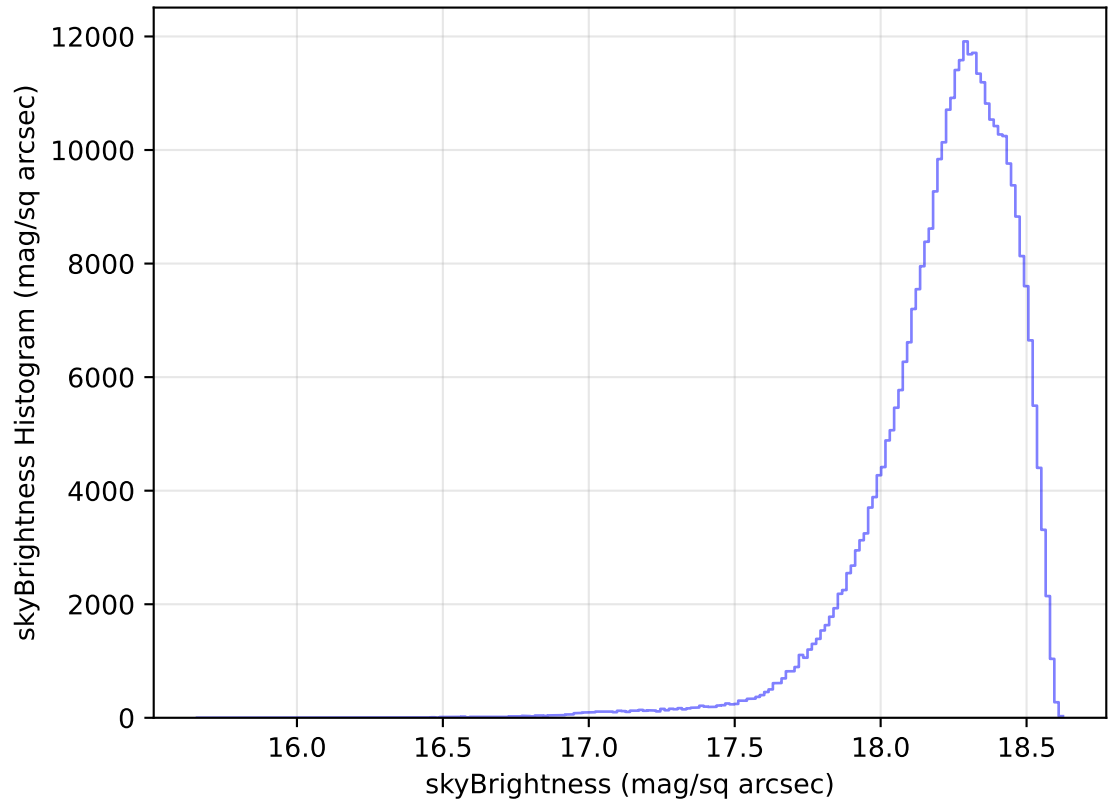
internal_u_expt30_nscale1.2v3.4_10yrs WFD y band: skyBrightness Histogram
