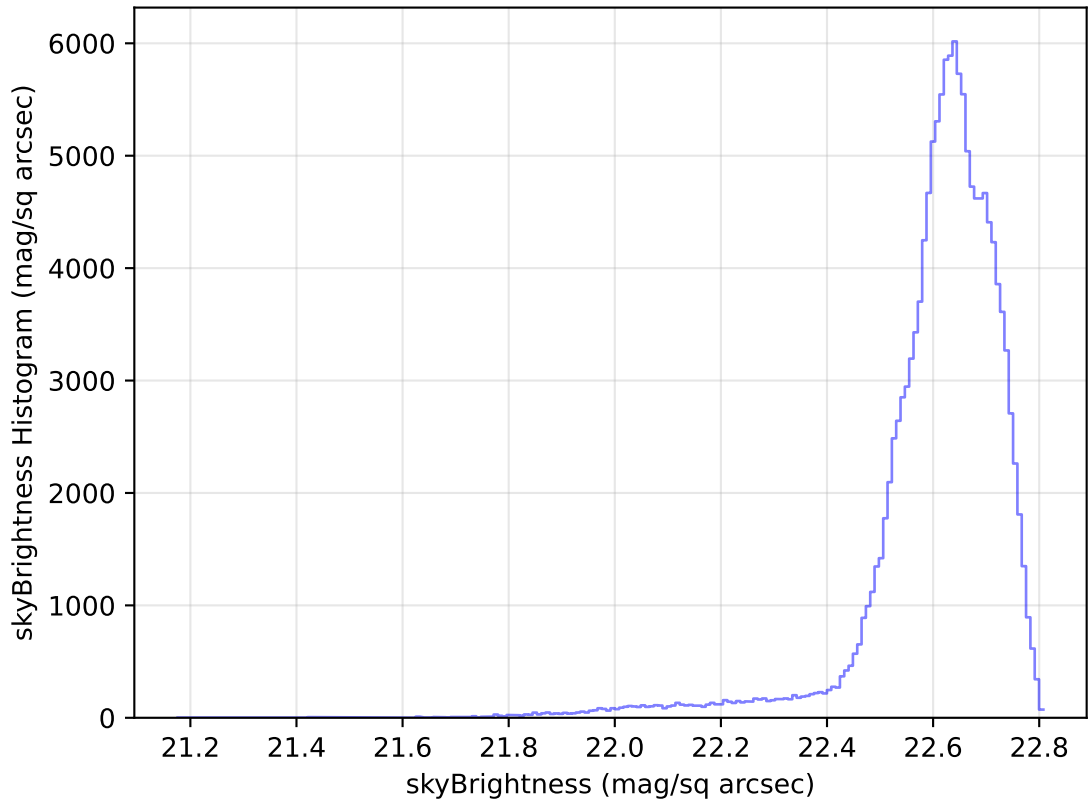
internal_u_expt30_nscale1.2v3.4_10yrs WFD u band: skyBrightness Histogram
