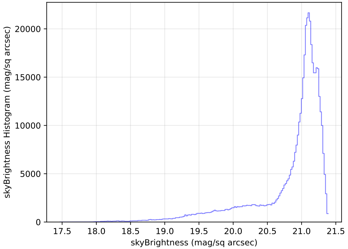
internal_u_expt30_nscale1.2v3.4_10yrs WFD r band: skyBrightness Histogram
