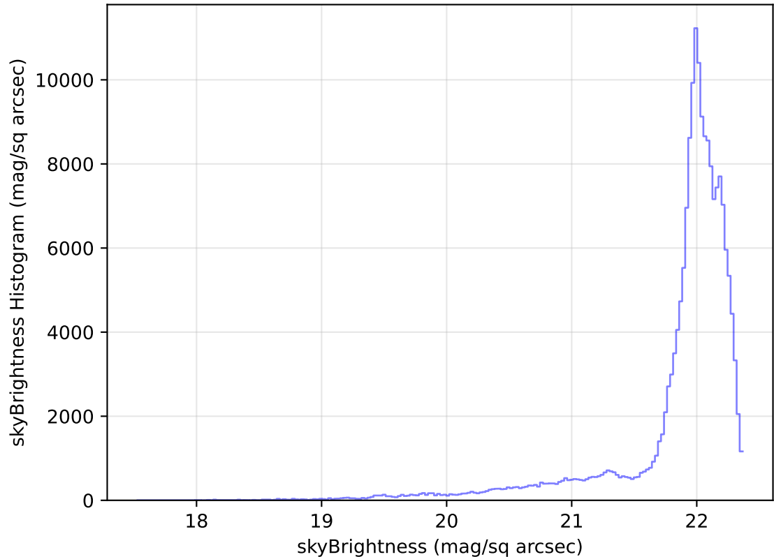
internal_u_expt30_nscale1.2v3.4_10yrs WFD g band: skyBrightness Histogram
