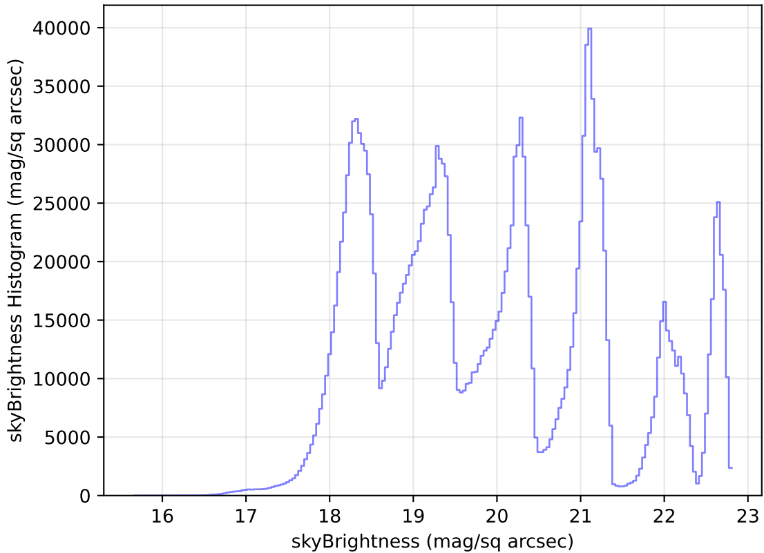
internal_u_expt30_nscale1.2v3.4_10yrs WFD all bands: skyBrightness Histogram
