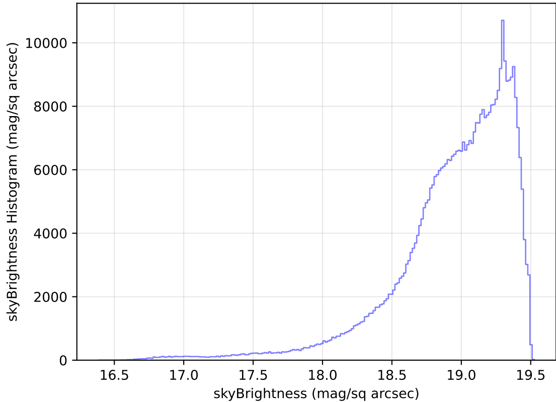
internal_u_expt30_nscale1.2v3.4_10yrs All sky z band: skyBrightness Histogram
