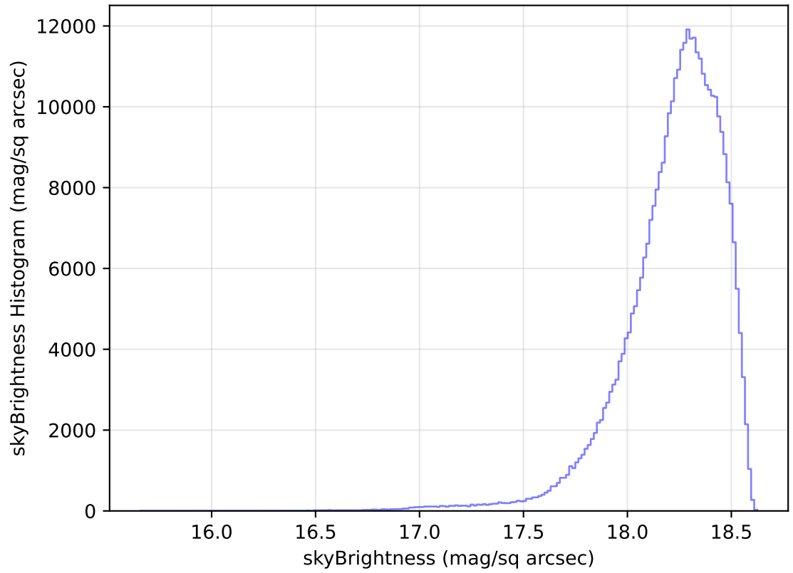
internal_u_expt30_nscale1.2v3.4_10yrs All sky y band: skyBrightness Histogram
