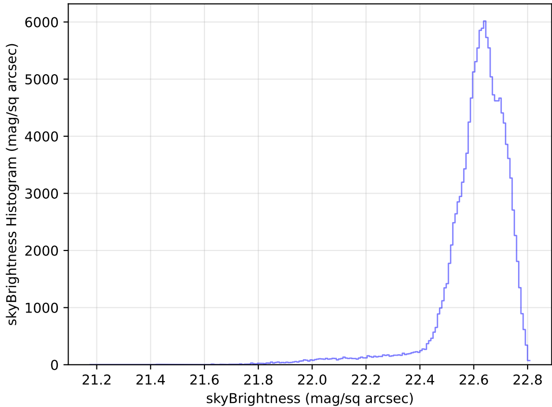
internal_u_expt30_nscale1.2v3.4_10yrs All sky u band: skyBrightness Histogram
