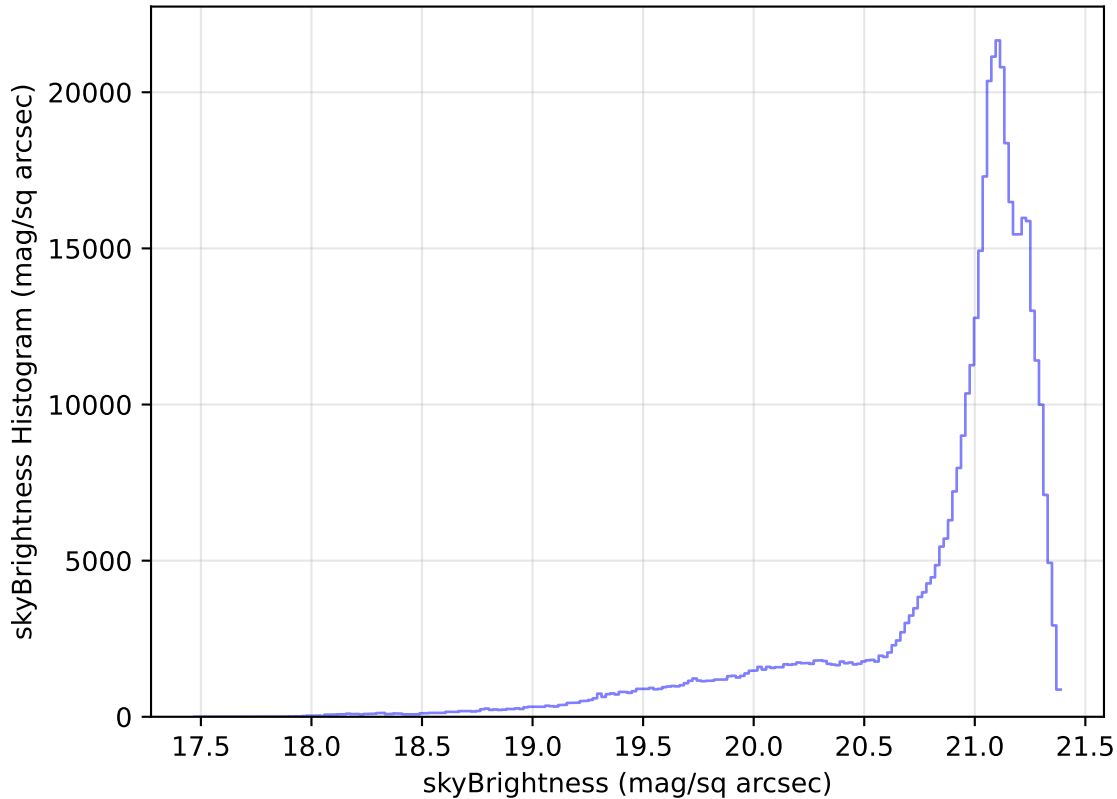
internal_u_expt30_nscale1.2v3.4_10yrs All sky r band: skyBrightness Histogram
