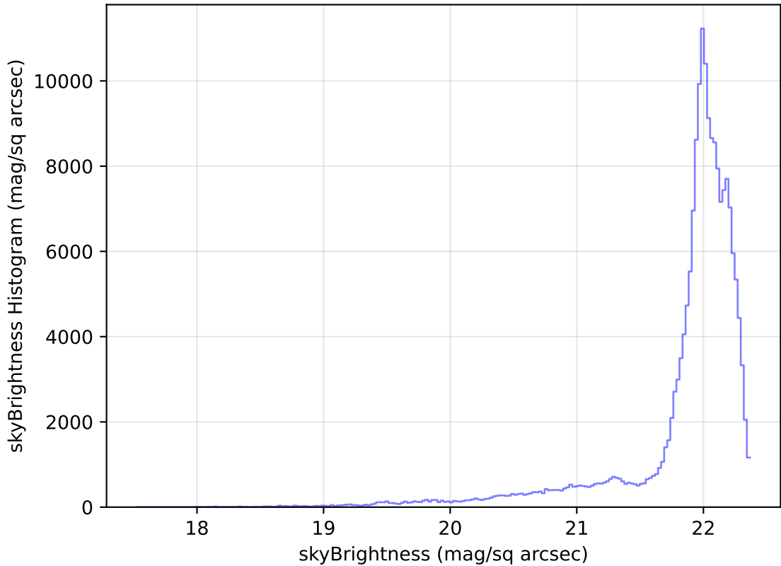
internal_u_expt30_nscale1.2v3.4_10yrs All sky g band: skyBrightness Histogram
