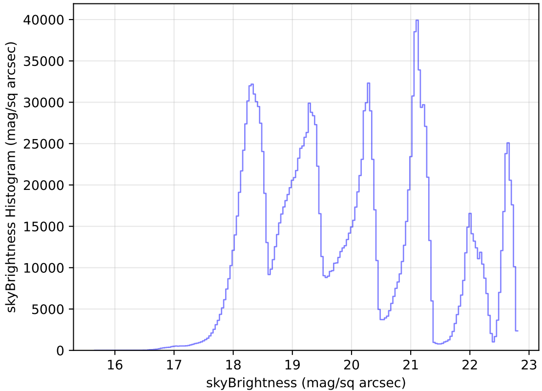
internal_u_expt30_nscale1.2v3.4_10yrs All sky all bands: skyBrightness Histogram
