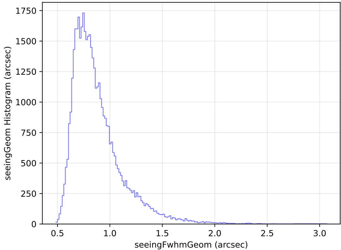
internal_u_expt30_nscale1.2v3.4_10yrs Yr 1 z band: seeingGeom Histogram
