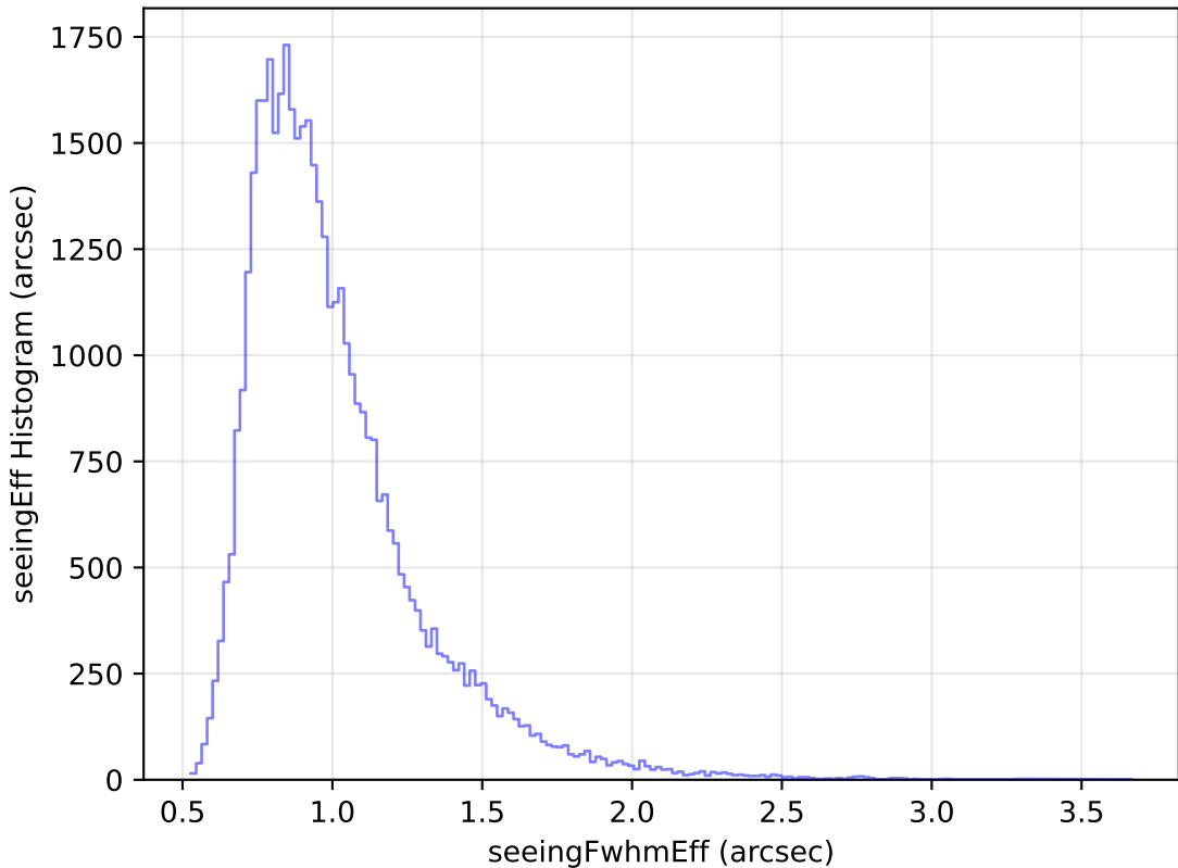
internal_u_expt30_nscale1.2v3.4_10yrs Yr 1 z band: seeingEff Histogram
