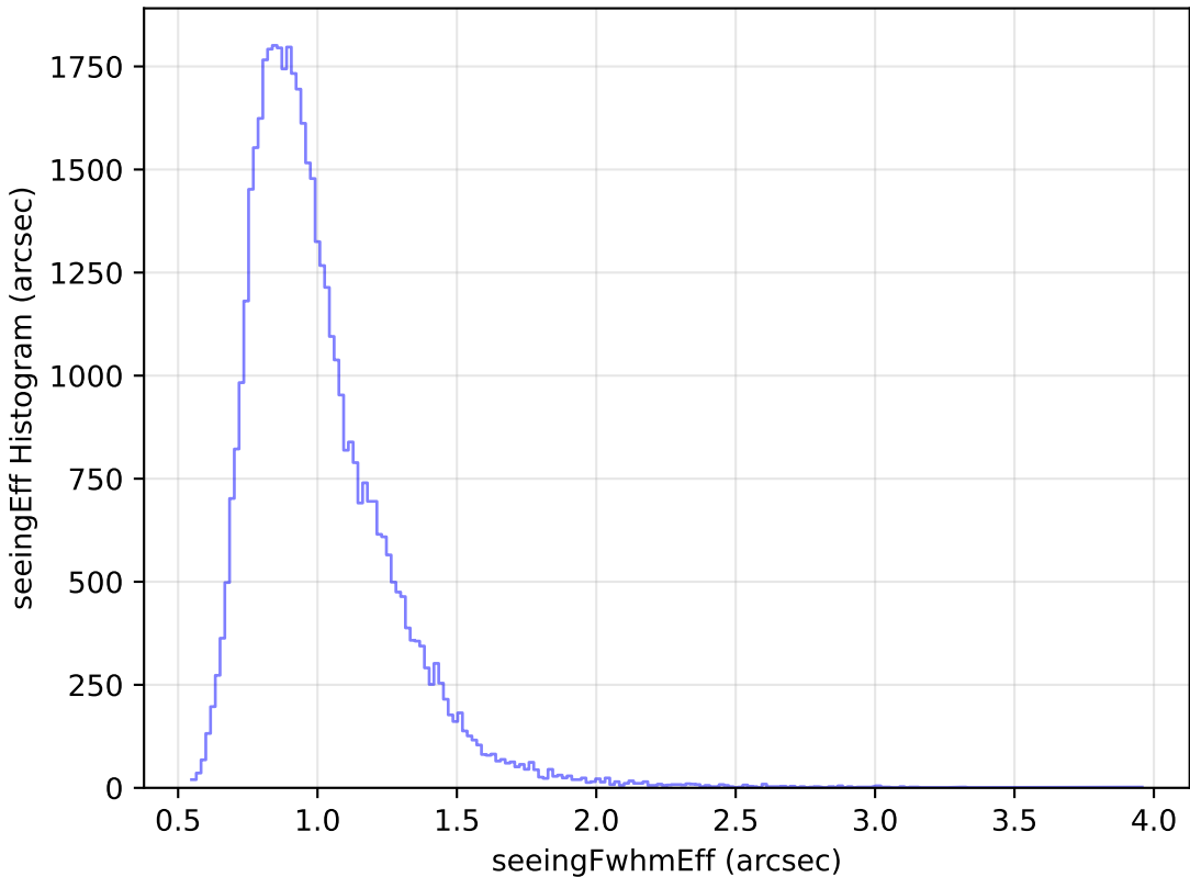
internal_u_expt30_nscale1.2v3.4_10yrs Yr 1 y band: seeingEff Histogram
