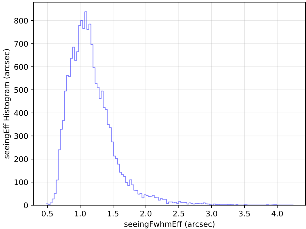
internal_u_expt30_nscale1.2v3.4_10yrs Yr 1 u band: seeingEff Histogram
