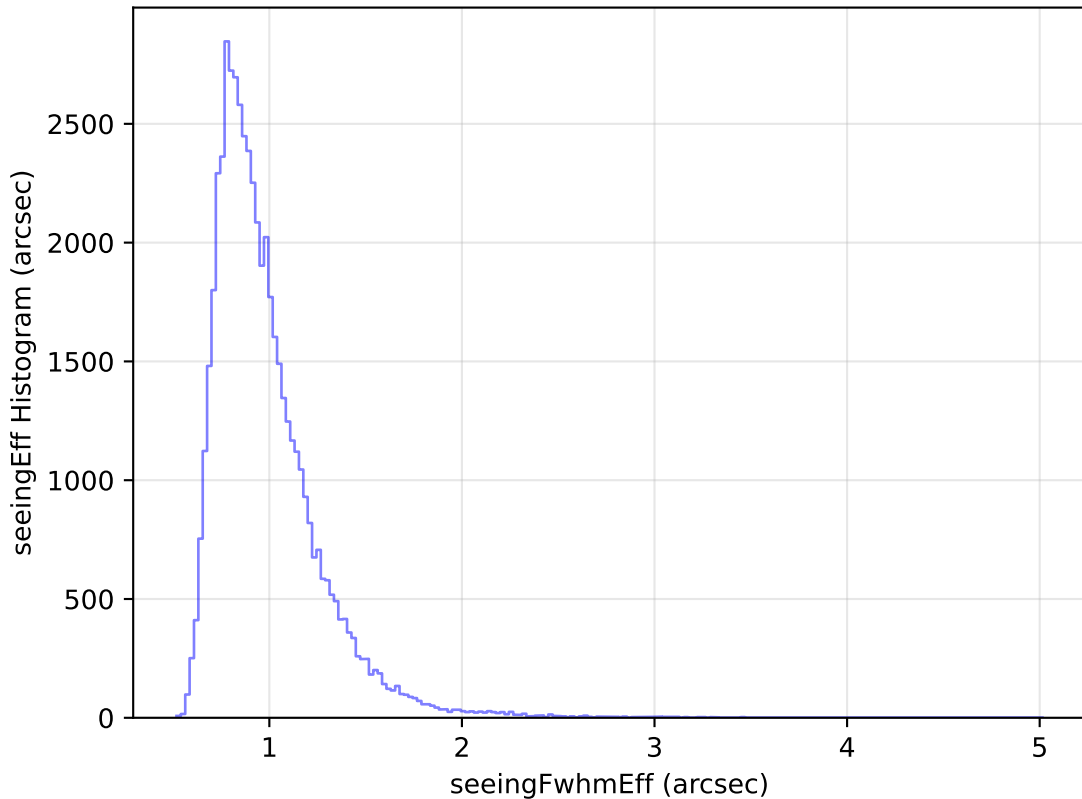
internal_u_expt30_nscale1.2v3.4_10yrs Yr 1 i band: seeingEff Histogram
