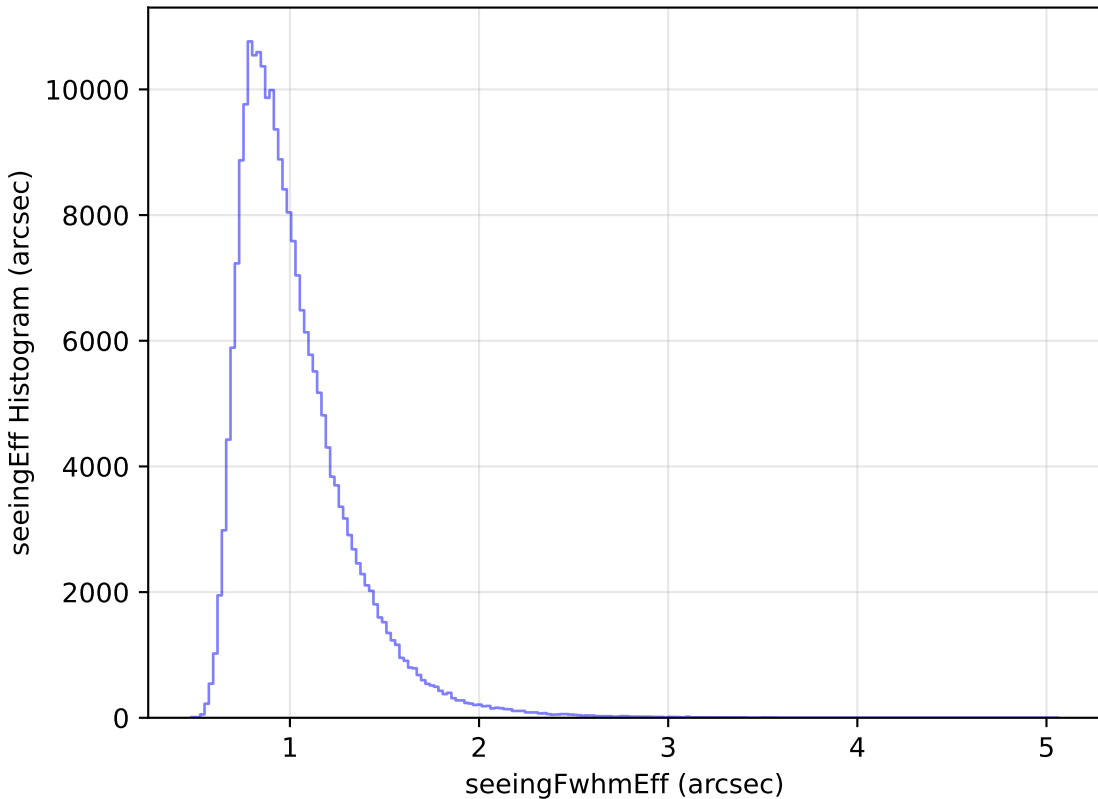
internal_u_expt30_nscale1.2v3.4_10yrs Yr 1 all bands: seeingEff Histogram
