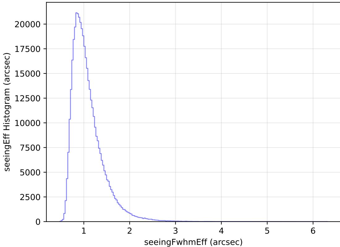
internal_u_expt30_nscale1.2v3.4_10yrs WFD z band: seeingEff Histogram
