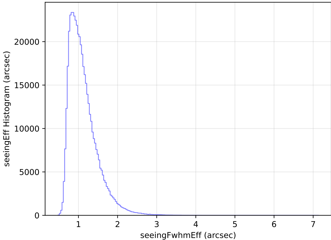
internal_u_expt30_nscale1.2v3.4_10yrs WFD r band: seeingEff Histogram
