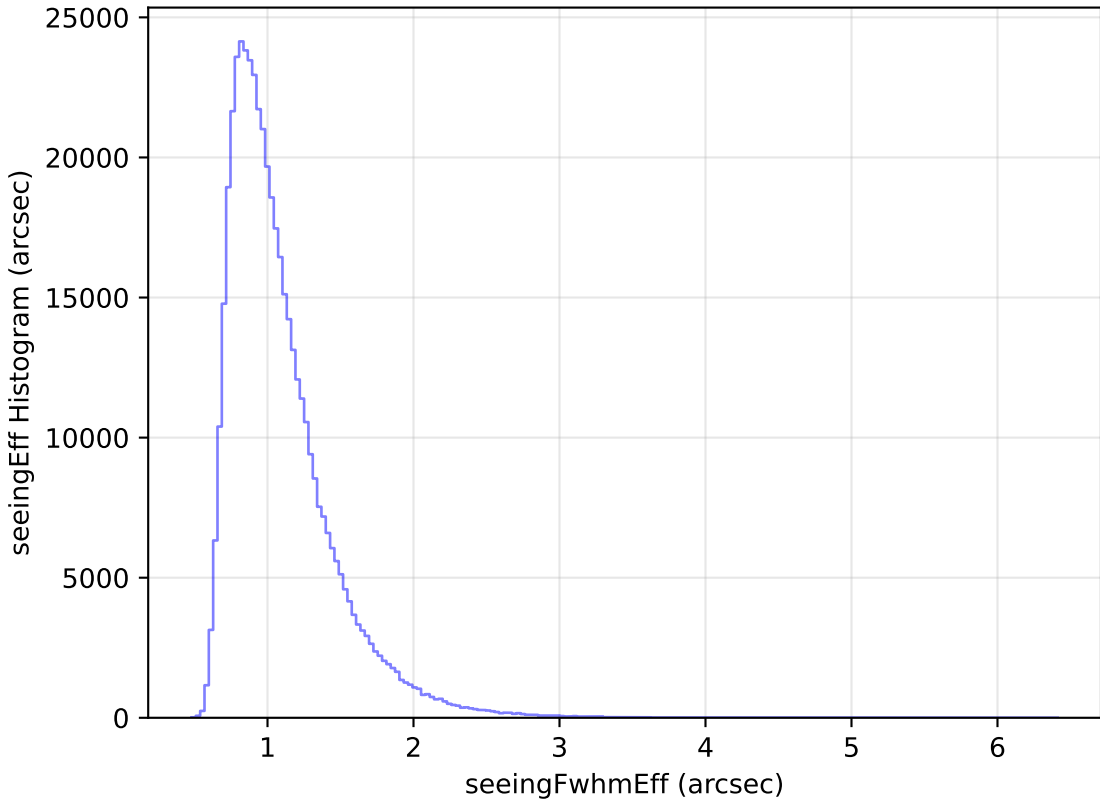
internal_u_expt30_nscale1.2v3.4_10yrs WFD i band: seeingEff Histogram
