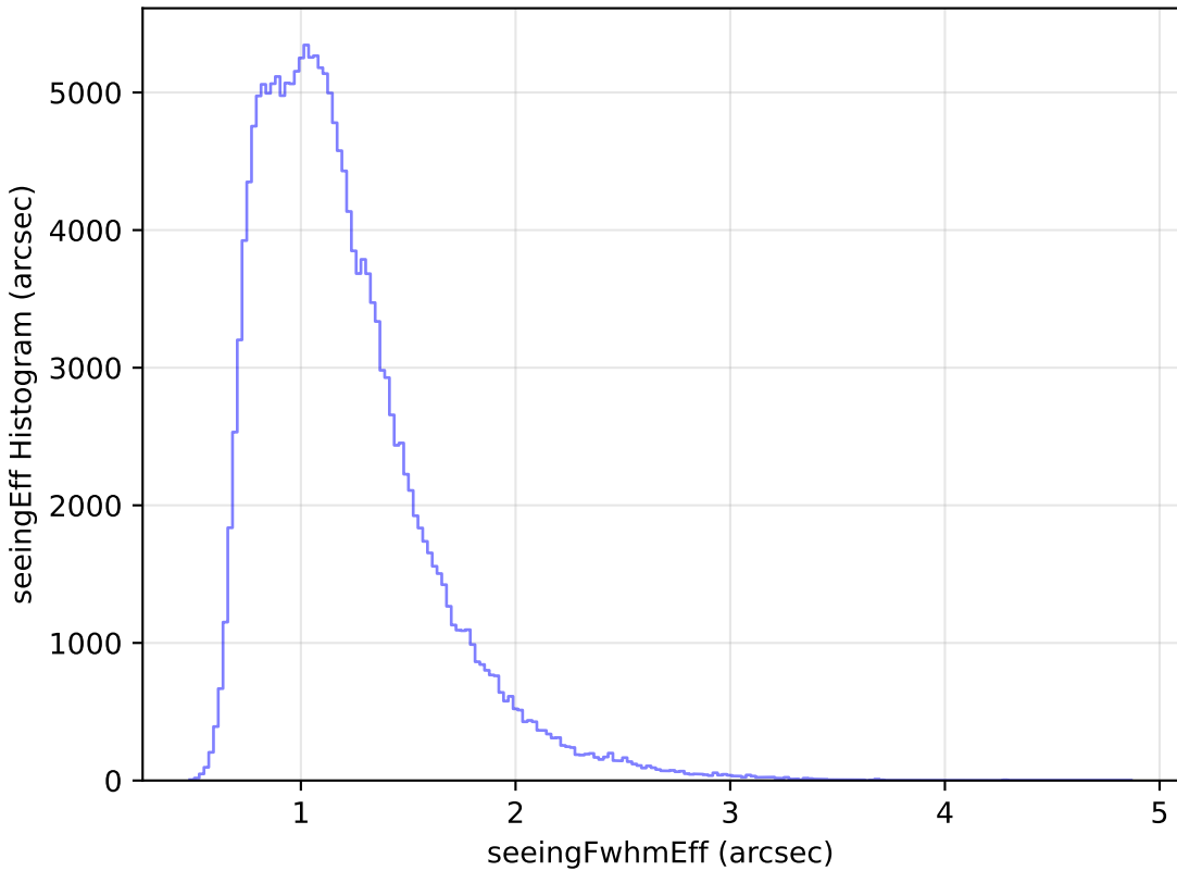
internal_u_expt30_nscale1.2v3.4_10yrs WFD g band: seeingEff Histogram
