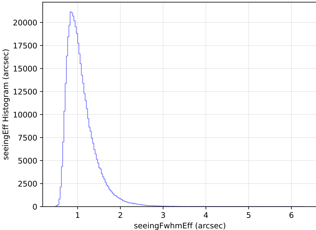
internal_u_expt30_nscale1.2v3.4_10yrs All sky z band: seeingEff Histogram
